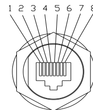
Figure 3.4 RS485 pin of R5series
