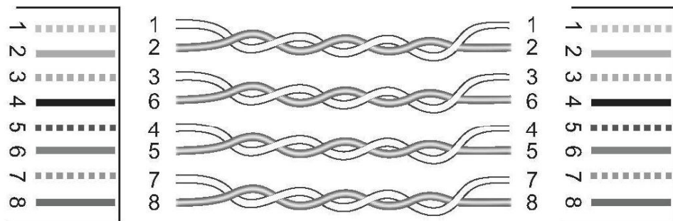
Connection diagram of crosstalk line pair
