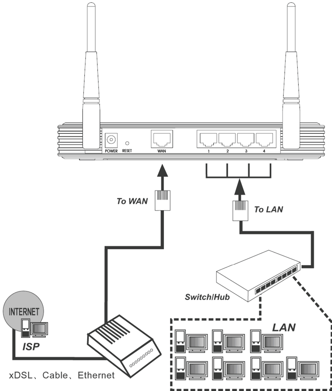
Figure 2-1 Hardware Installation of the TL-WR841ND Wireless N Router
