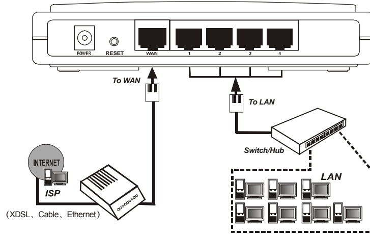
Figure 3-1 Hardware Installation of the TL-R402M Cable/DSL Router
