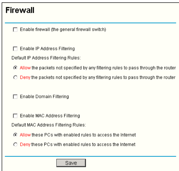
Figure 5-19 Firewall Settings
