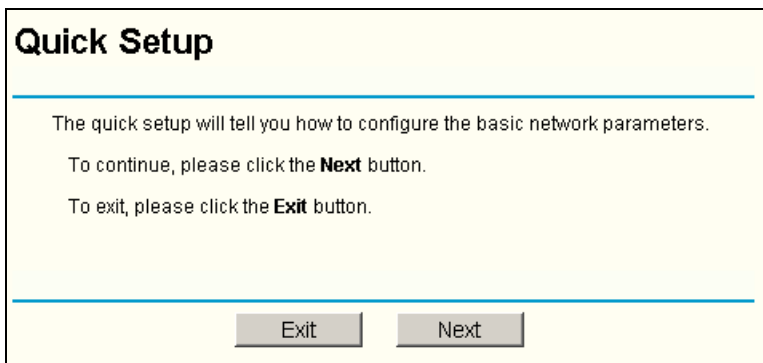
Figure 4-5 Quick Setup
