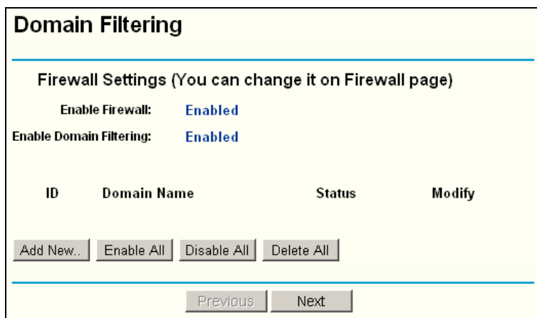
Figure 5-22 Domain Filtering
