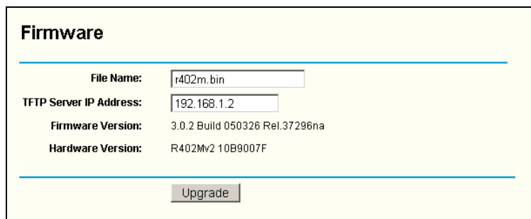
Figure 5-30 Firmware Upgrade
