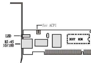
Figure 1 PCI Fast Ethernet Adapter
